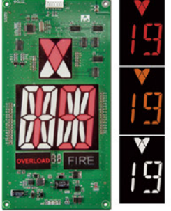
SM.04HL16/B Optional Display: Segment Display Color: Red, Orange, White Installation: Vertical Size: 213.4×109.2×19.9
