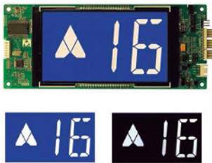
SM.04HL16/D Optional Display Size: 5.7" Display: White on blue White on Black Installation: Horizontal Size: 218×86.2×9.4
