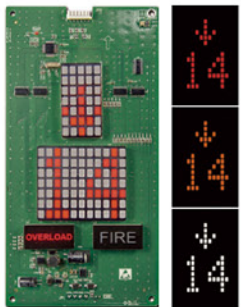
SM.04VR/13 Optional Display: Dotmatrix Display Color: Red, Orange, White Installation: Vertical Size: 231.4×109.2×20
