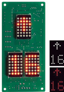
SM.04VR/K Standard Display: Dotmatrix Display Color: Red, White Installation: Vertical Size: 183×70×25
