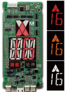
SM.04HL16/AE Optional Display: Segment Display Color: Red, Orange, White Installation: Vertical Size: 162.5×72×8
