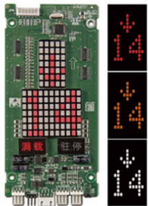
SM.04VR/12 Optional Display: Dotmatrix Display Color: Red, Orange, White Installation: Vertical Size: 162.5×72×7.7
