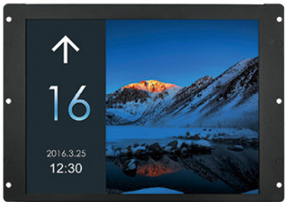
SM.04TL/H(Pictures) SM.04TL/P(Video) Optional Display Size: 10.4" Display: TFT Resolution: 800×600 Size: 253.2×179.2×41
