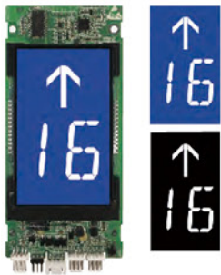
SM.04VL16/XE Optional Display Size: 4.3" Display: White on blue White on Black Installation: Vertical Size: 162.4×72×8.5
